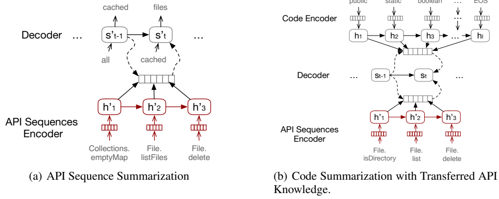
Figure 2: The model of TL-CodeSum
