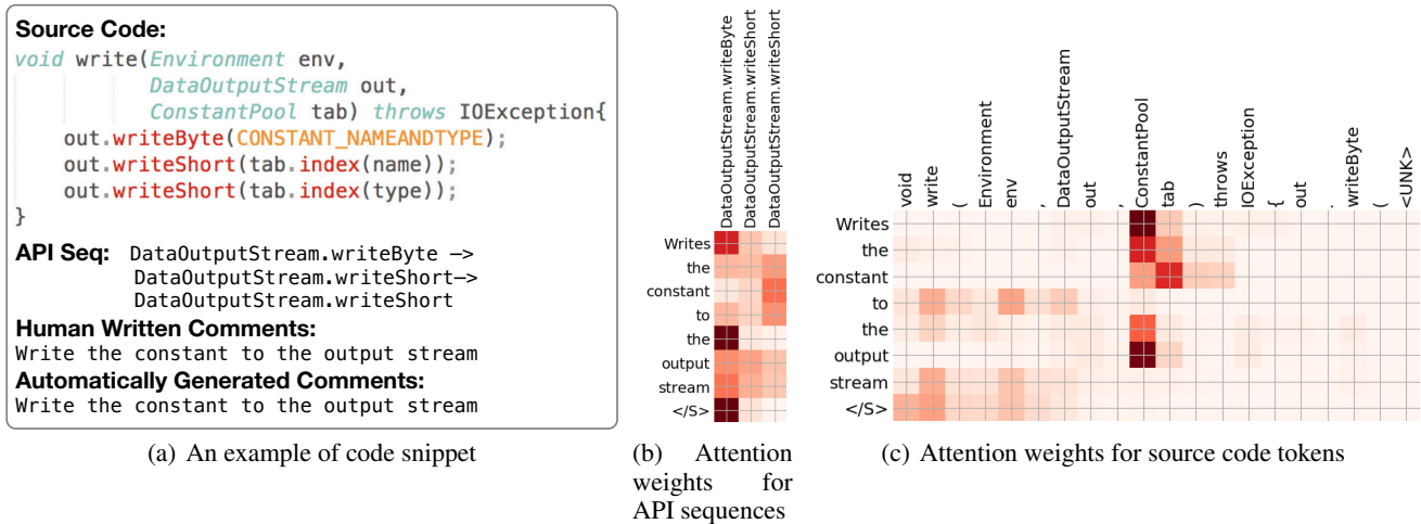
Figure 4: Heatmap of attention weights for API sequence and source code snippets. The model learns to align key summary words with the corresponding tokens in API sequences and source code.
